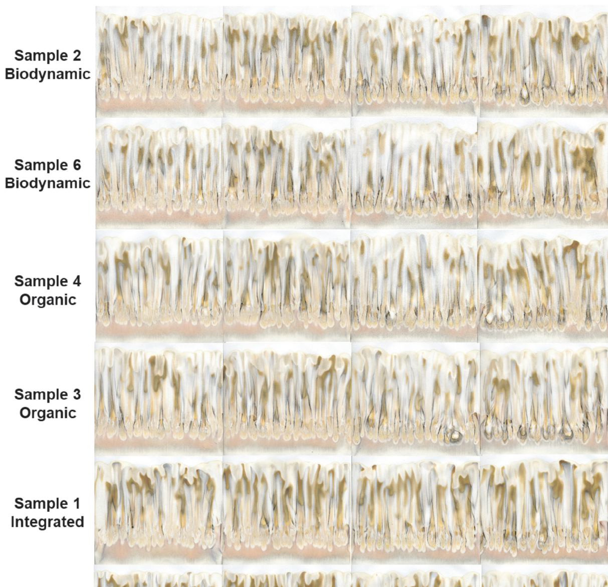
Figure S1. Six samples from biodynamic, organic and integrated management systems: capillary dynamolysis images of grape juice pressed with the standard procedure at Geisenheim harvest year 2007 (juice aged 1 days at 5 °C; images 0.30, 0.35, 0.40, 0.45 ml juice)
