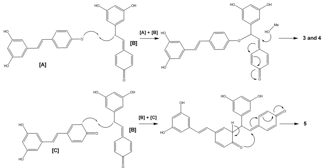
FIGURE S5. Hypotheses for the formation of resveratrol dimers.
