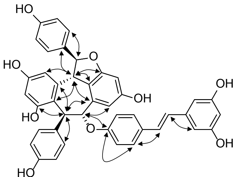
FIGURE S2. Main HMBC correlations of compound 7.
