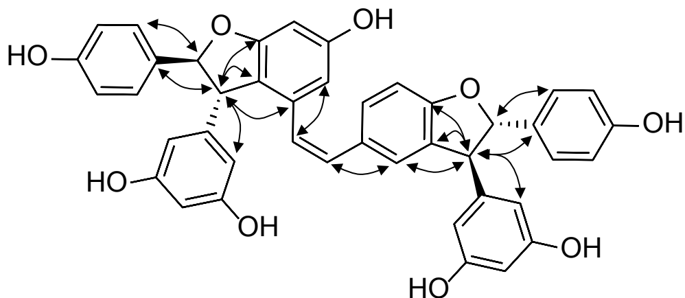
FIGURE S4. Main HMBC correlations of compound 10.
