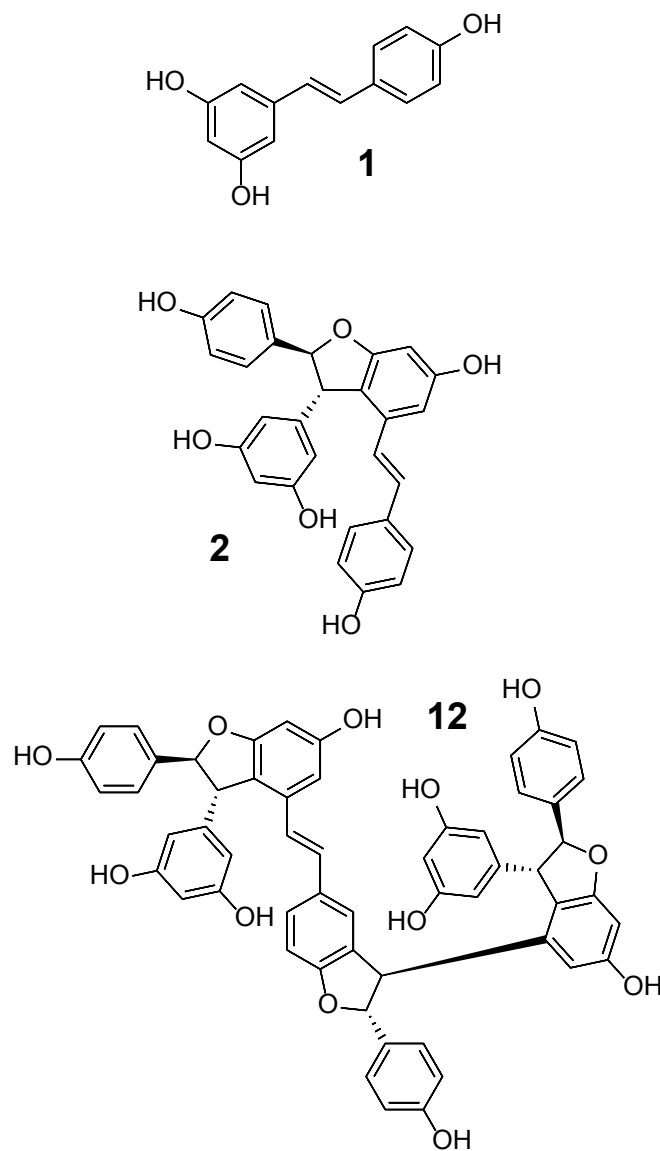
FIGURE S1. Structures of the main constituents of the extract CE.
