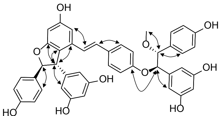
FIGURE S3. Main HMBC correlations of compound 9.
