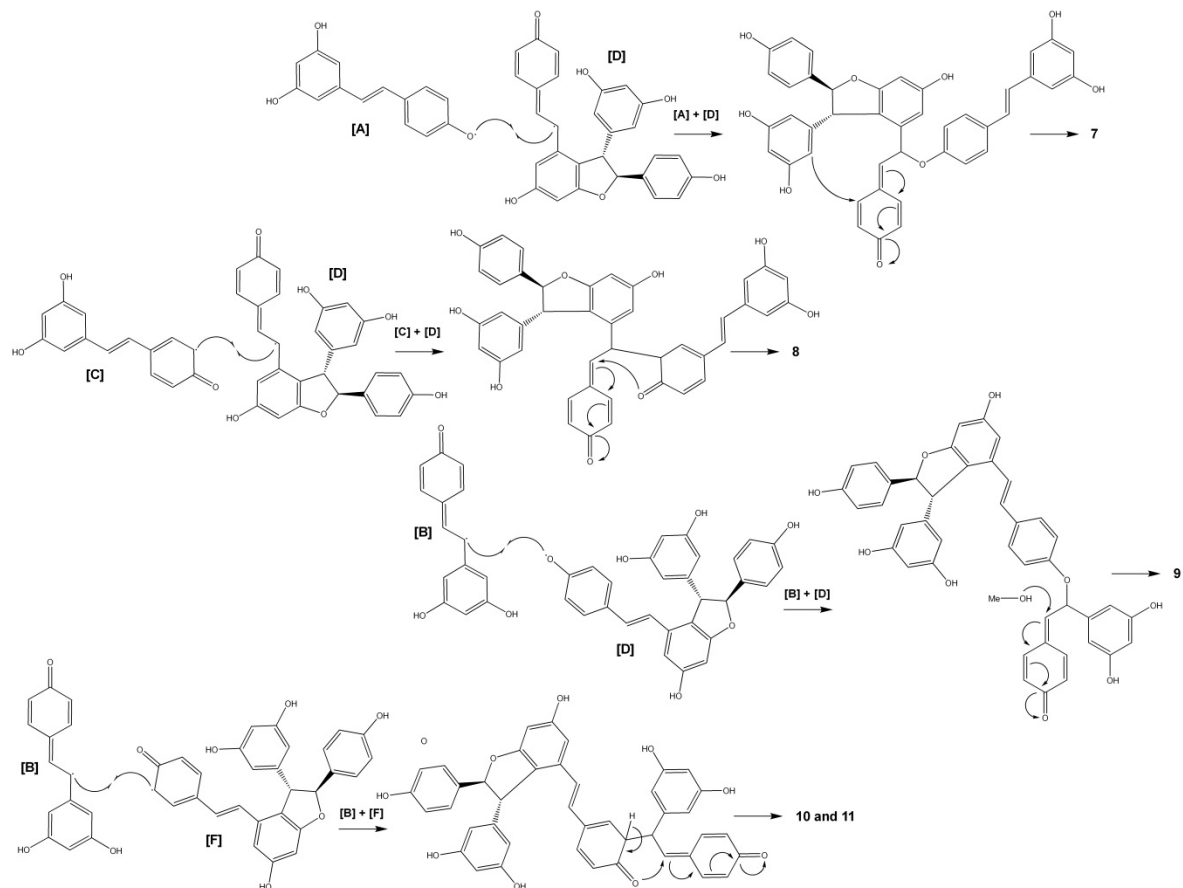
FIGURE S6. Hypotheses for the formation of resveratrol trimers.
