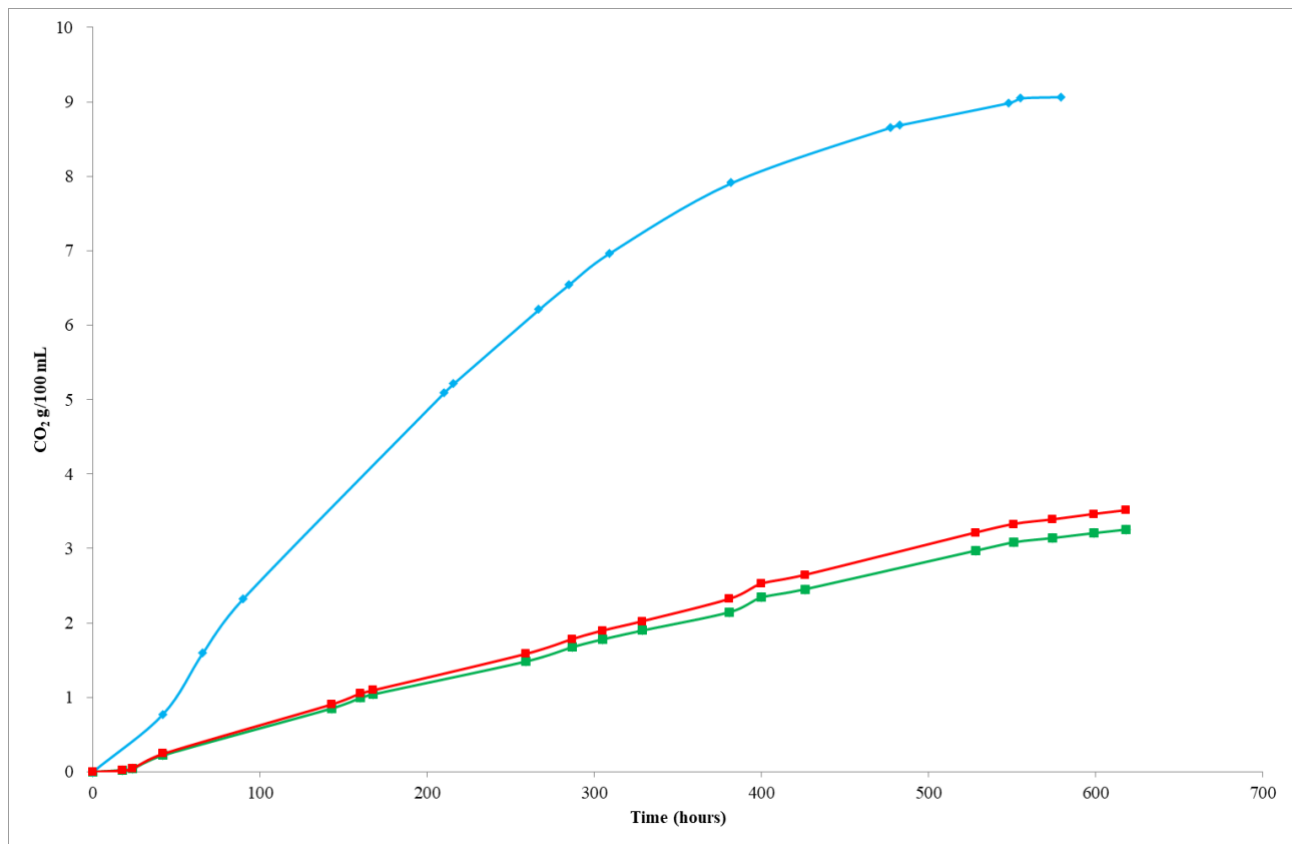
Supplementary Figure 1. Fermentation (CO 2 released/time) in synthetic must of S. cerevisiae EC1118 (—) and S. bacillaris FRI751 (—) and PAS13 (—) strains.
