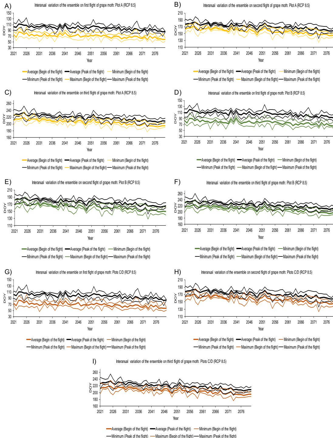
FIGURE S3. Chronograms of the interannual variation (DOY) of the beginning and peak of each LB flight (three flights) in the period 2021-2080 at each plot (A, B and C/D) in the RCP8.5 scenario.
