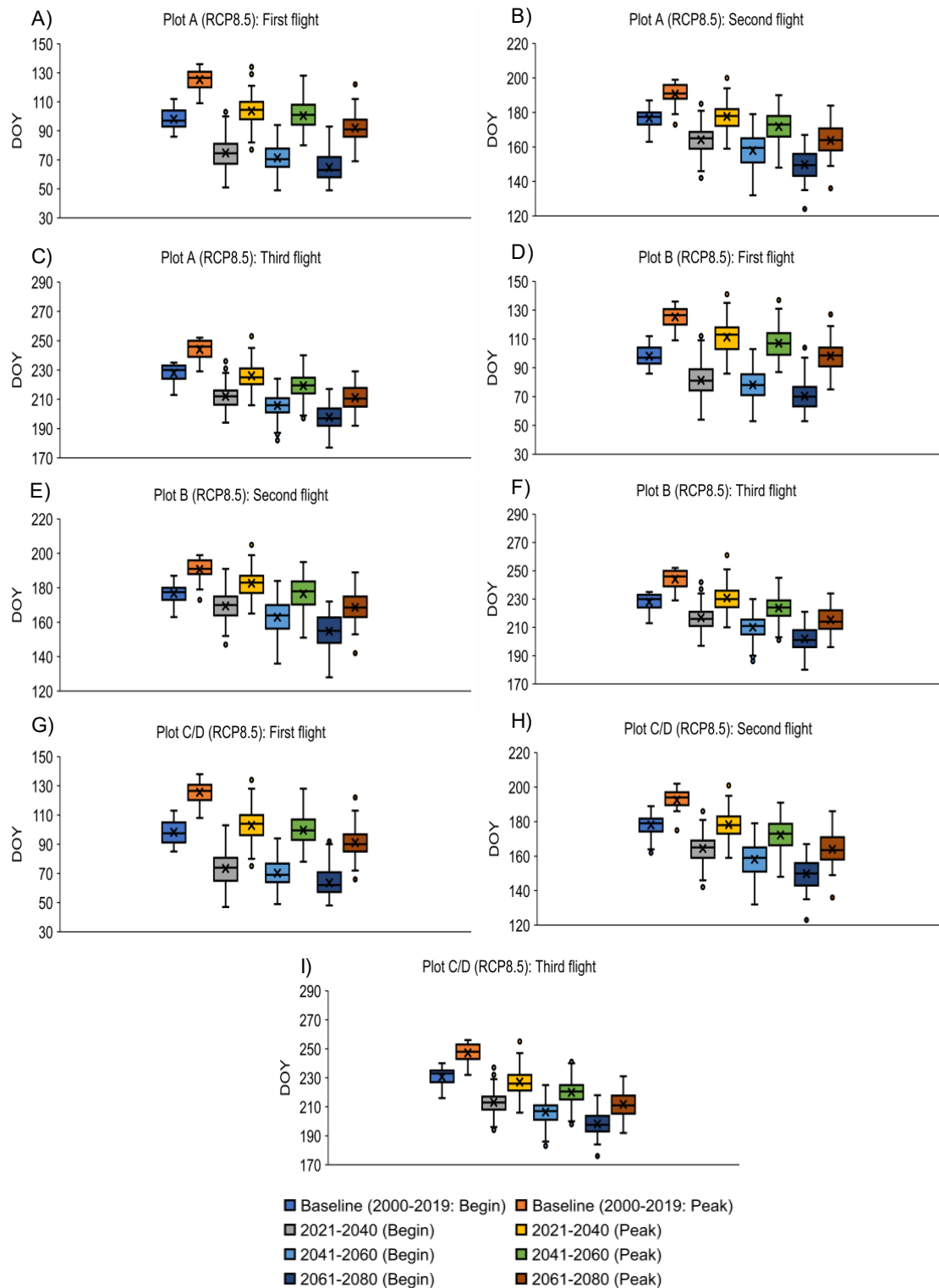
FIGURE S1. Box-plot diagrams of the beginning and peak of the LB first, second and third flights for the outlined plots (A, B, C and D) over baseline (2000-2019), the short-term (2021–2040), medium-term (2041–2060) and long-term (2061–2080) periods under RCP8.5. See legend for details. The × represents the average, the solid line within the boxes the median. The box upper (lower) limit corresponds to the third (first) quartile, while the whiskers correspond to the non-outlier extremes. Outliers (black circles) are considered as values above (below) the box upper (lower) limit by a factor of 1.5 IQR (Interquartile Range, i.e. box height).
