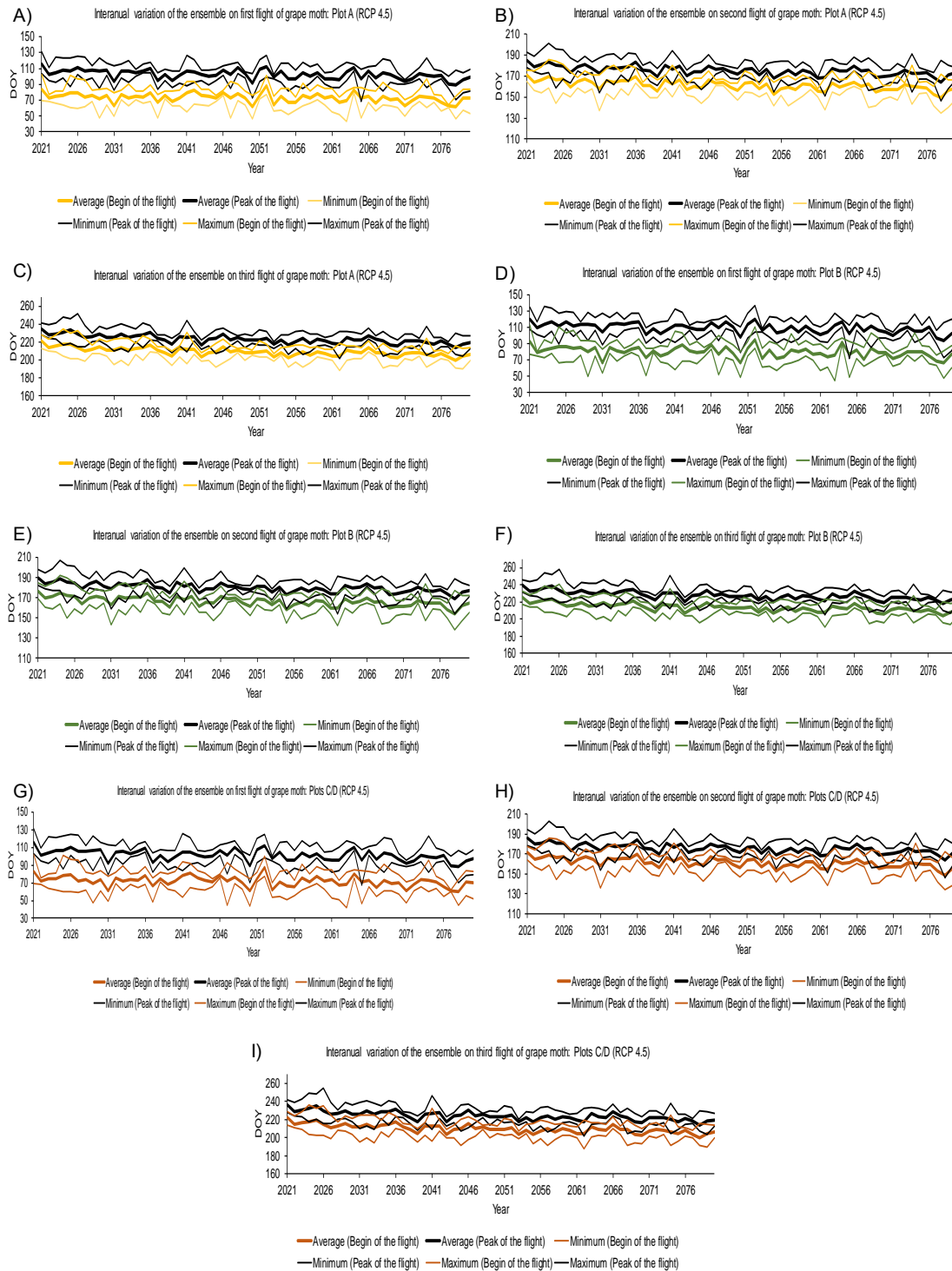
FIGURE S2. Chronograms of the interannual variation of the beginning and peak dates (DOY) of each LB flight (three flights) in the period 2021-2080 at each plot (A, B and C/D) in the RCP4.5 scenario.
