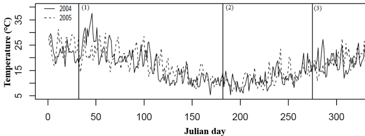
Figure S1. Seasonal changes in daily mean temperatures (2004 and 2005). Vertical lines represent 1 February (1, Julian day 32), 1 July (2, Julian day 182) and 1 October (3, Julian day 275).
