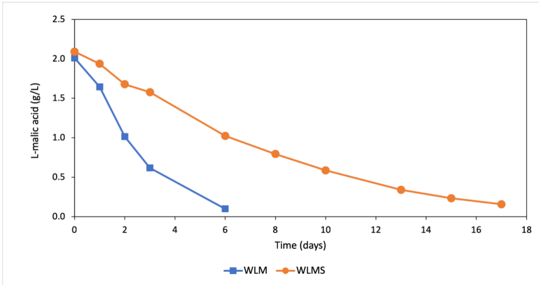
Figure S1. Consumption of L-malic acid by O. oeni PSU-1 in the control condition without succinic acid (WLM) and with 2 g/L of succinic acid (WLMS). Values are the means of triplicates; error bars are not visible because all were lower than 0.01.
